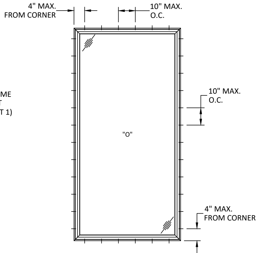
ANCHOR LAYOUT THROUGH FRAME INSTALLATION
