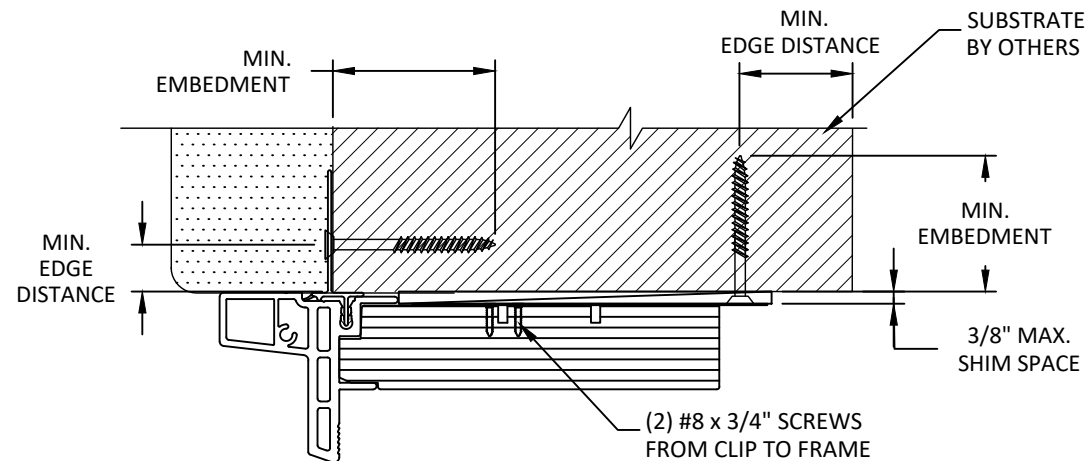
A/5 VERTICAL SECTION THROUGH INSTALLATION CLIP & NAIL FIN HEAD/JAMB/SILL
